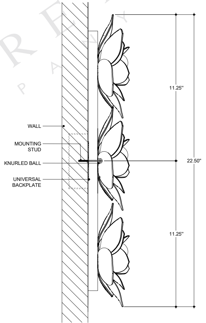
SIDE VIEW
